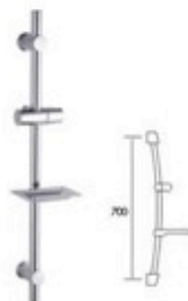
SD1005 ABS brackets, chrome plating ABS slider, chrome plating Stainless steel sliding bar Transparent soap dish Dimension: L:700, D:25
