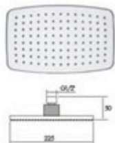
SU1014 Model: overhead shower Material: ABS Size: 225x150x50mm
