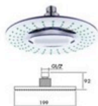
SU1012 Model: overhead shower Material: ABS Size: 199x199x92mm Color:
