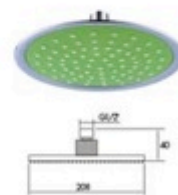
SU1022 Model: overhead shower Material: ABS Size: 208x208x40mm Color:
