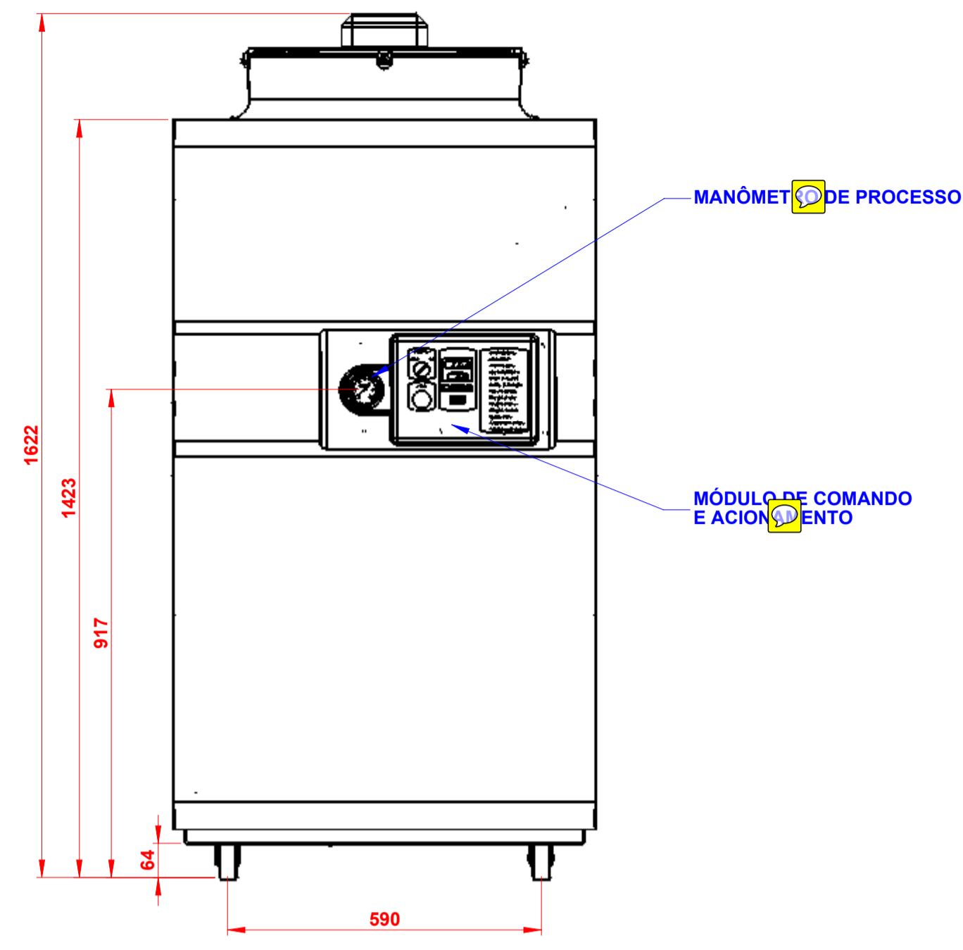
VISTA LANTAL
