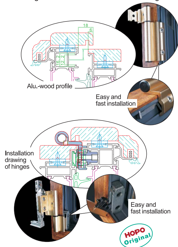
ATT90---Patent tilt-turn fitting for Alu-wood profile. 16mm U groove combined with 14-18mm C groove.
