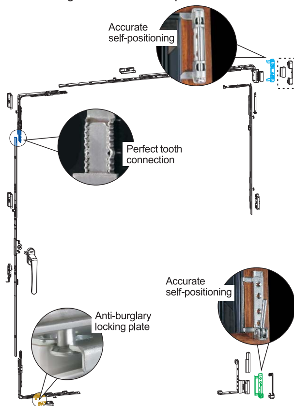
Tilt-turn fitting for wood and PVC profiles made of SS304
