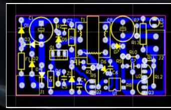
electronic driver
